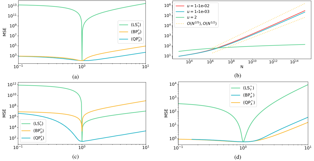
Fig. 1: (a, c, d) Average losses plotted on a log-log scale with respect to the normalized parameter. (a) Low-noise regime PI of (LS_r^*) (b) Low-noise regime PI of (QP_\lambda^*) , R^\#(u\lambda^*; s, N) computed analytically as a function of N [11, Prop 15] (c) Very sparse regime PI of (BP_\sigma^*) (d) Parameter stability regime.
